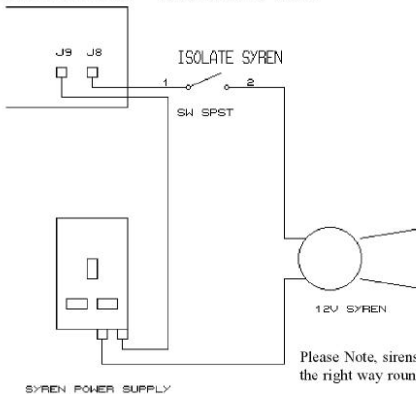
DIACONS CONTROL BOX With External Siren
